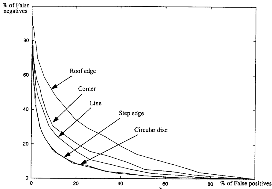
Figure 8. A comparison of feature detection rates for our five example features. All results are for SNR = 1.0 and for a disc shaped window containing 49 pixels. We see that the step edge and circular disc are less noise sensitive than the other features. Note however that the noise sensitivity of all features may be reduced by increasing the size of the window. Further, for SNR around 3.0 and above, all the feature detectors perform with very little error.
