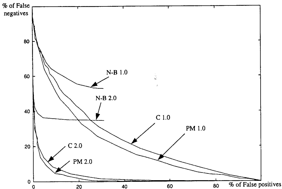
Figure 7. A comparison of edge detection rates. The Canny (C), Nalwa-Binford (N-B), and parametric manifold (PM) detectors are compared for SNR = 1.0 and 2.0. We plot false positives against false negatives. For each detector and SNR, the result is a curve parameterized by the threshold inherent in that detector. The closer a curve lies to the origin, the better the performance. We see that the Canny detector and the parametric manifold technique perform comparably. The results for the Nalwa-Binford detector are consistent with those presented in (Nalwa and Binford, 1986) but are of a fundamentally different nature. See text for a discussion of this.
