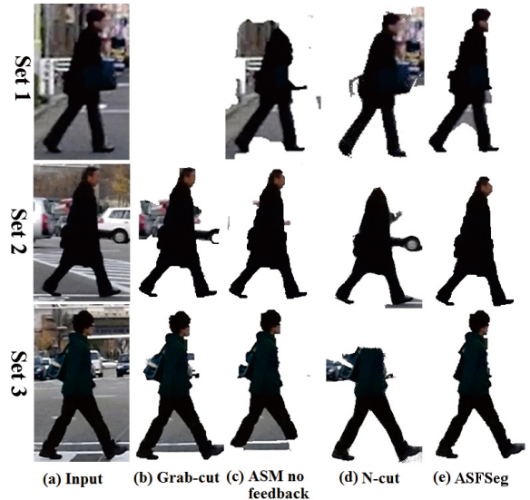
Figure 5. Comparison between the segmentations by Grab-cut, N-cut and ASFSeg methods. The images have been resized for better presentation. Actual size is respectively: 82 \times 134 , 145 \times 206 and 138 \times 228 pixels.
